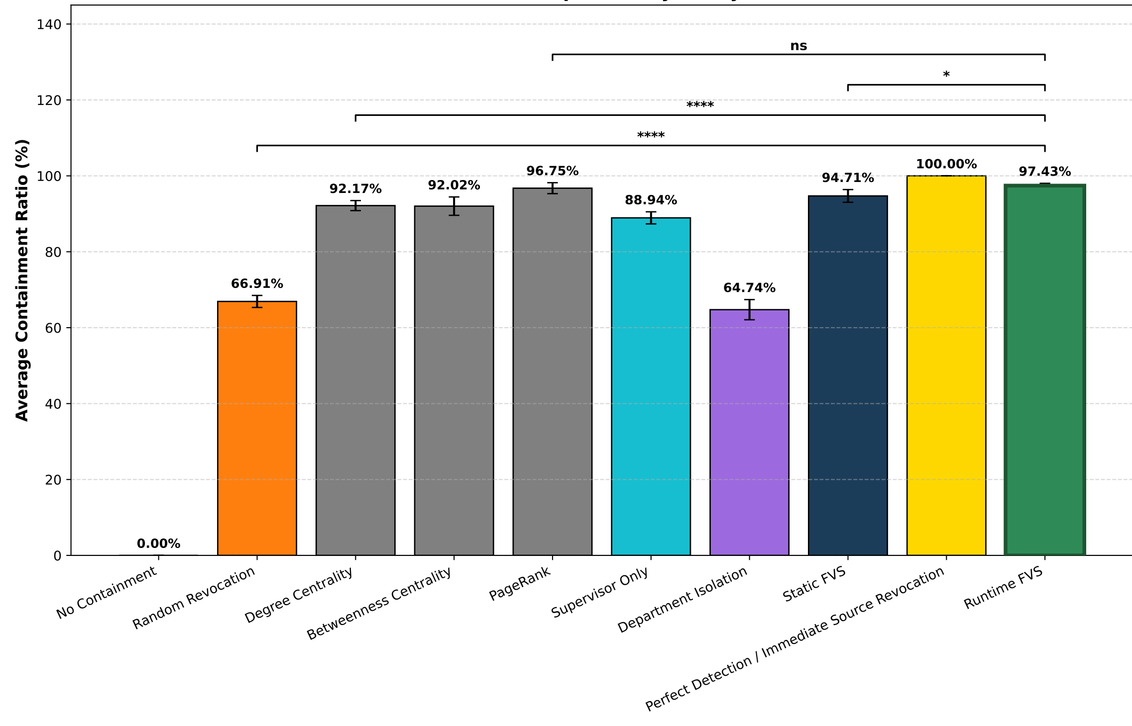
Containment Ratio Comparison by Policy (with 95% CI)
